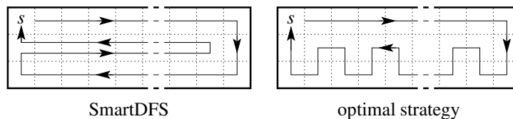
Figure 1.19: In a corridor of width 3 and with even length the bound S(P) = \frac{4}{3}S_{Opt}(P) - 2 holds.
