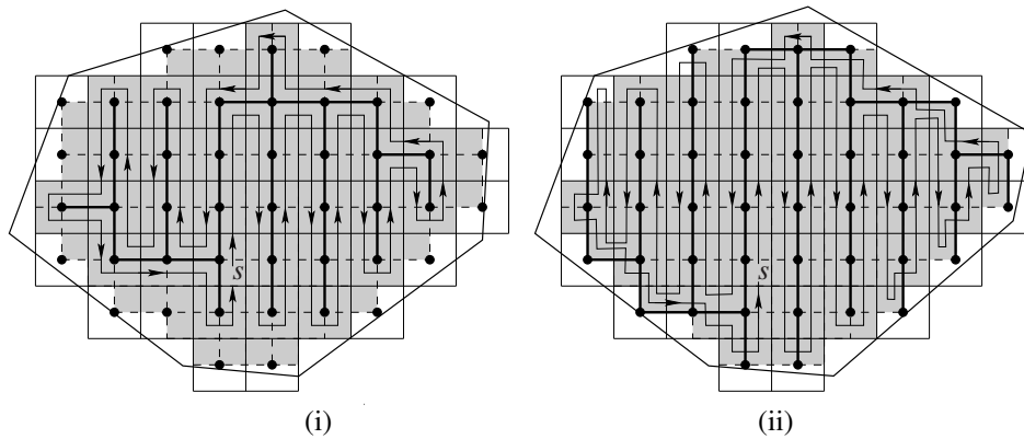
Figure 1.25: Example for (i) 2D-Scan-STC, (ii) Scan-STC.
